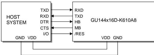
TTL Asynchronous serial communication from host system to VFD module.
