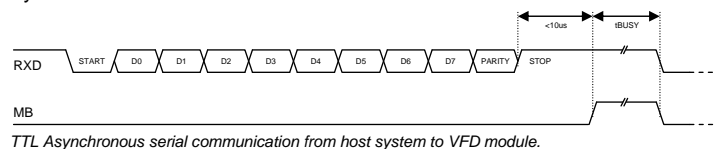
TTL Asynchronous serial communication from host system to VFD module.
