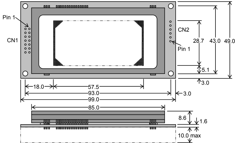
Dimensions in mm & subject to tolerances. Mounting holes 3.2mm dia.
