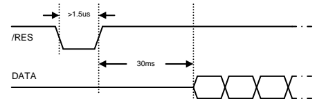
Reset timing diagram
