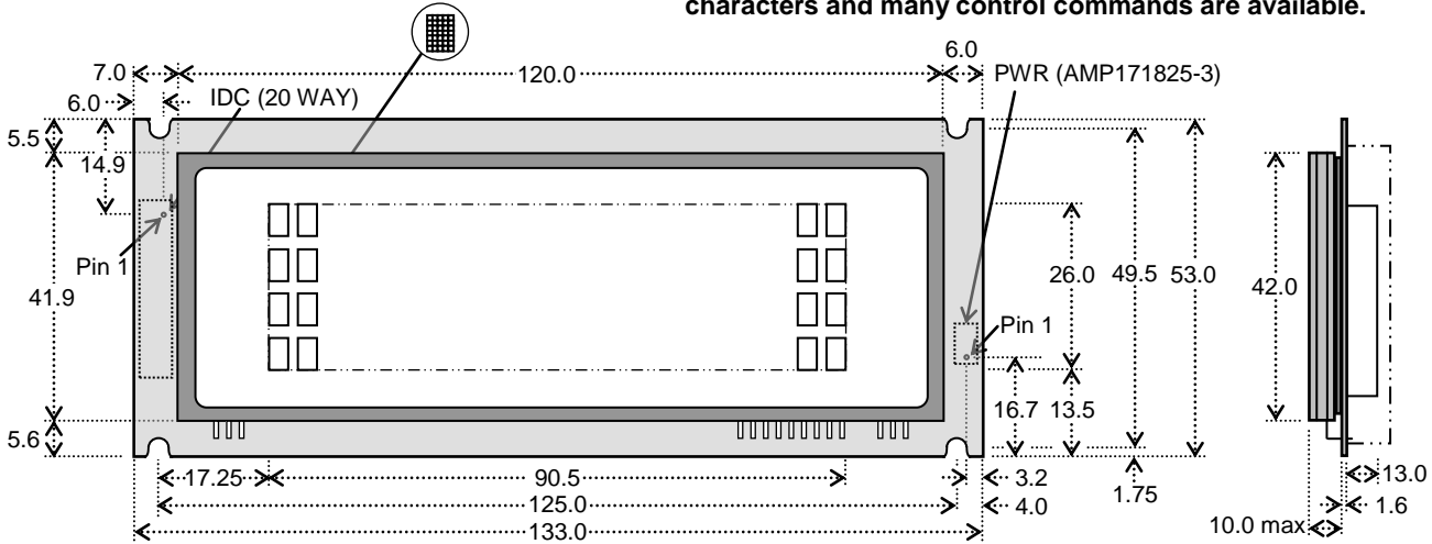
Dimensions in mm. Connector pitch is 2.54mm. See full spec for tolerances
