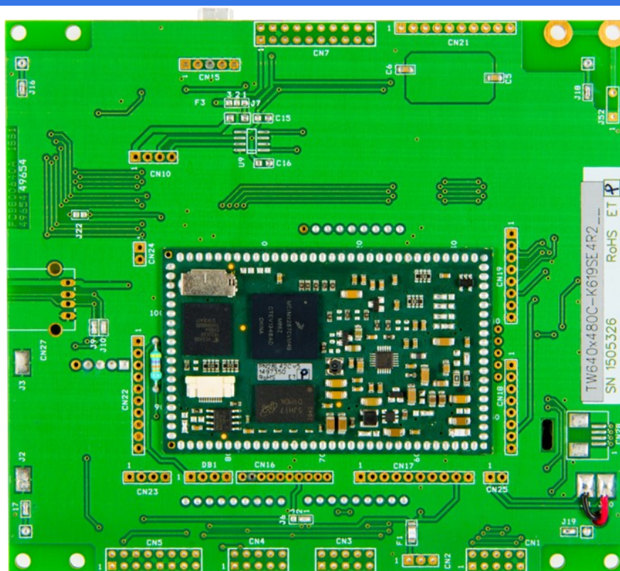
Figure 9 - TW640x480C- K619SE4R2RU Rear View
