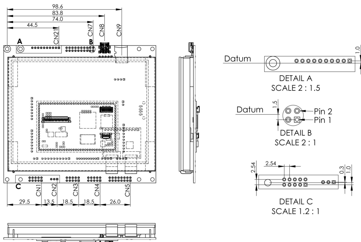
Figure 5- TW640x480C-K619SE4R2MU Connector Location drawing. Reference dimensions only.
