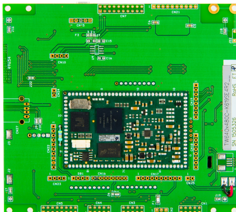
Figure 11 - TW640x480C- K619SE4R2NU Rear View
