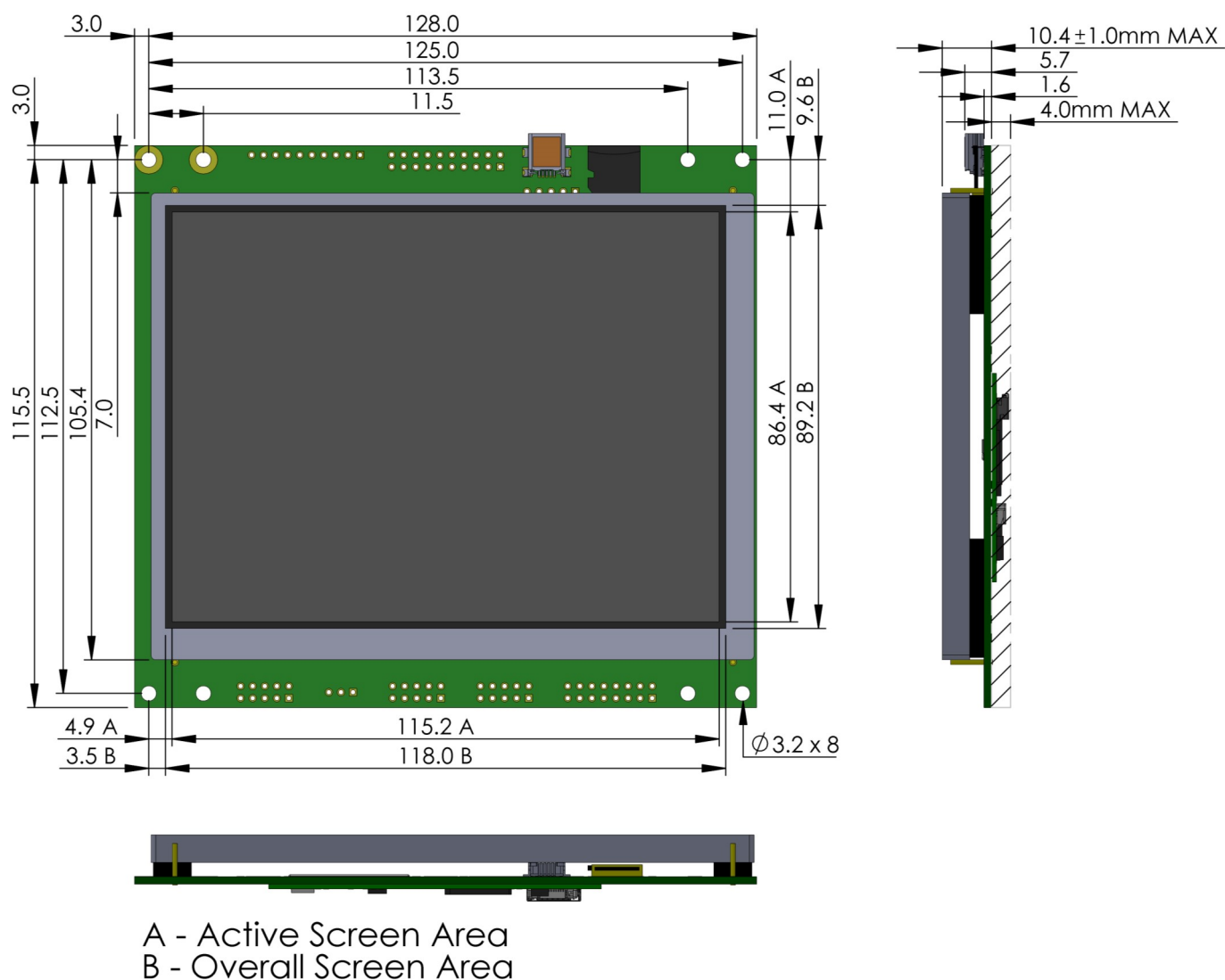
Figure 4 – TW640x480C-K619SE4R2NU Mechanical drawing. Reference dimensions only.
