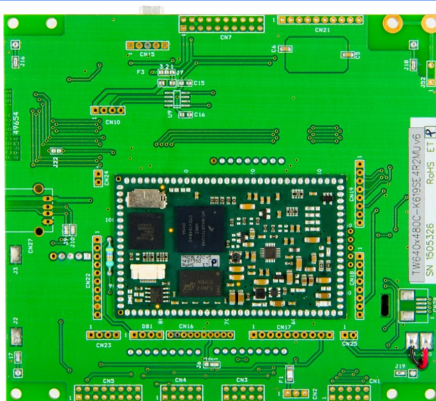
Figure 7 - TW640x480C- K619SE4R2MU Rear View
